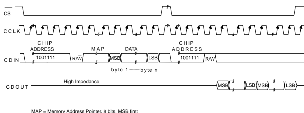
Figure 16. SPI Format
